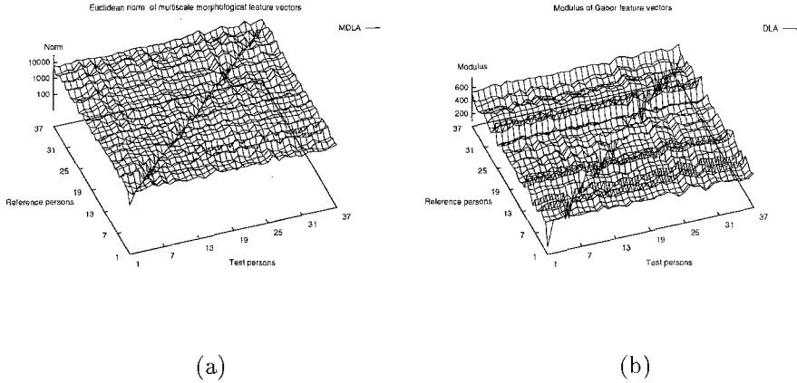
Fig. 4. Plots of elastic graph distances for all pairs of test and reference persons in MDLA and DLA. (a) Euclidean norm of multiscale morphological feature vectors. (b) Modulus of Gabor feature vectors.
