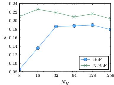
Figure 1. Effect of varying the number of codewords / RBF neurons ( N_K ) on the Cohen's \kappa metric (FI-2010 dataset)
