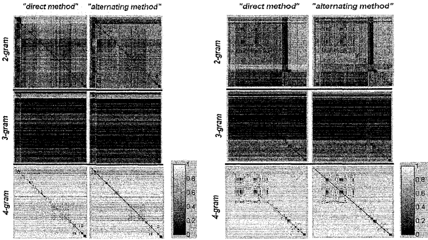
Fig. 1. Visualization of the matrices containing all the possible pairwise dissimilarities for the 497 proteins of Set1, for 2,3,4-gram models.
