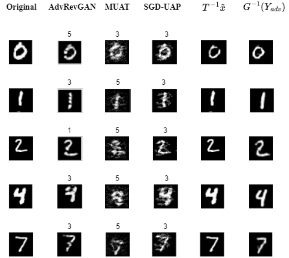
Fig. 2. Adversarial examples and reconstructed images on MNIST Dataset. The first column depicts original images \mathbf{x}_i , the next three columns are the corresponding adversarial examples \mathbf{y}_i^{adv} generated by the proposed method, MUAT and UAP respectively while above them demonstrated the wrong class that predicted by the model. In the last two columns are demonstrated the reconstructed images \mathbf{x}_i^{rec} derived by MUAT and our proposed method respectively.
